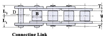
Connecting Link
