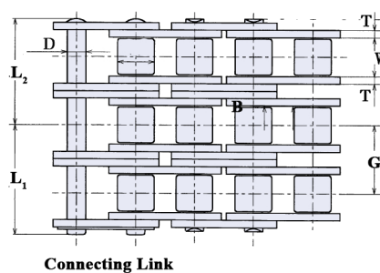
Connecting Link
