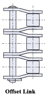
Offset Link
